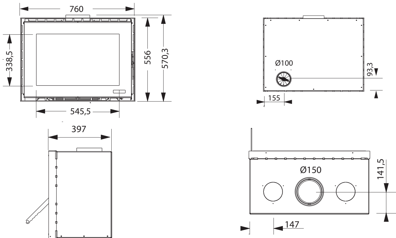
Inux 75 naturale / natural convection
